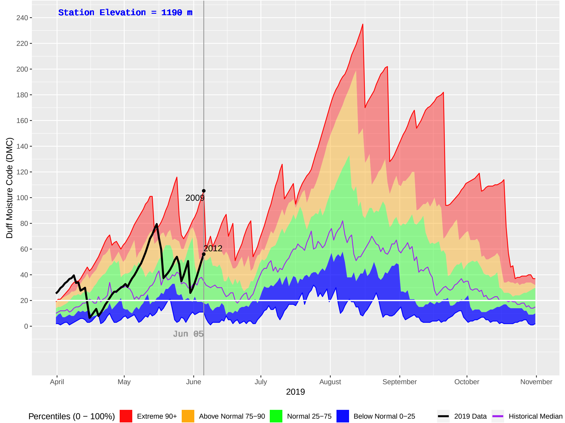
EMILY CREEK (425) : Historical (2002–2018), Current (2019) Daily Duff Moisture Code (DMC)
