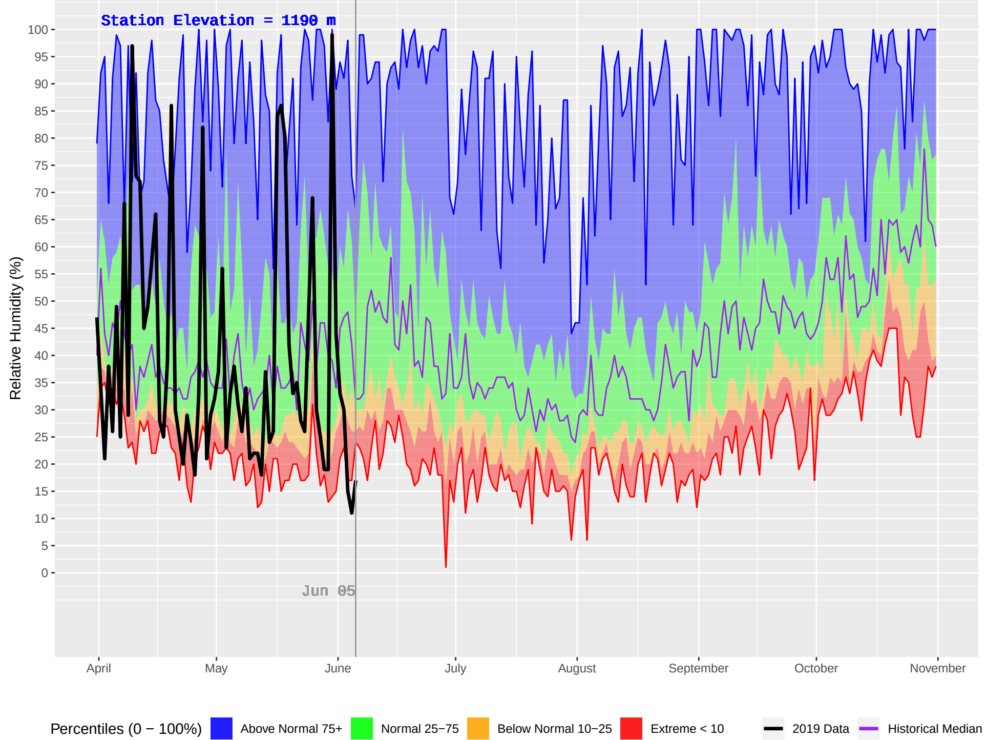
EMILY CREEK (425) : Historical (2002–2018) and Current (2019) Daily Relative Humidity
