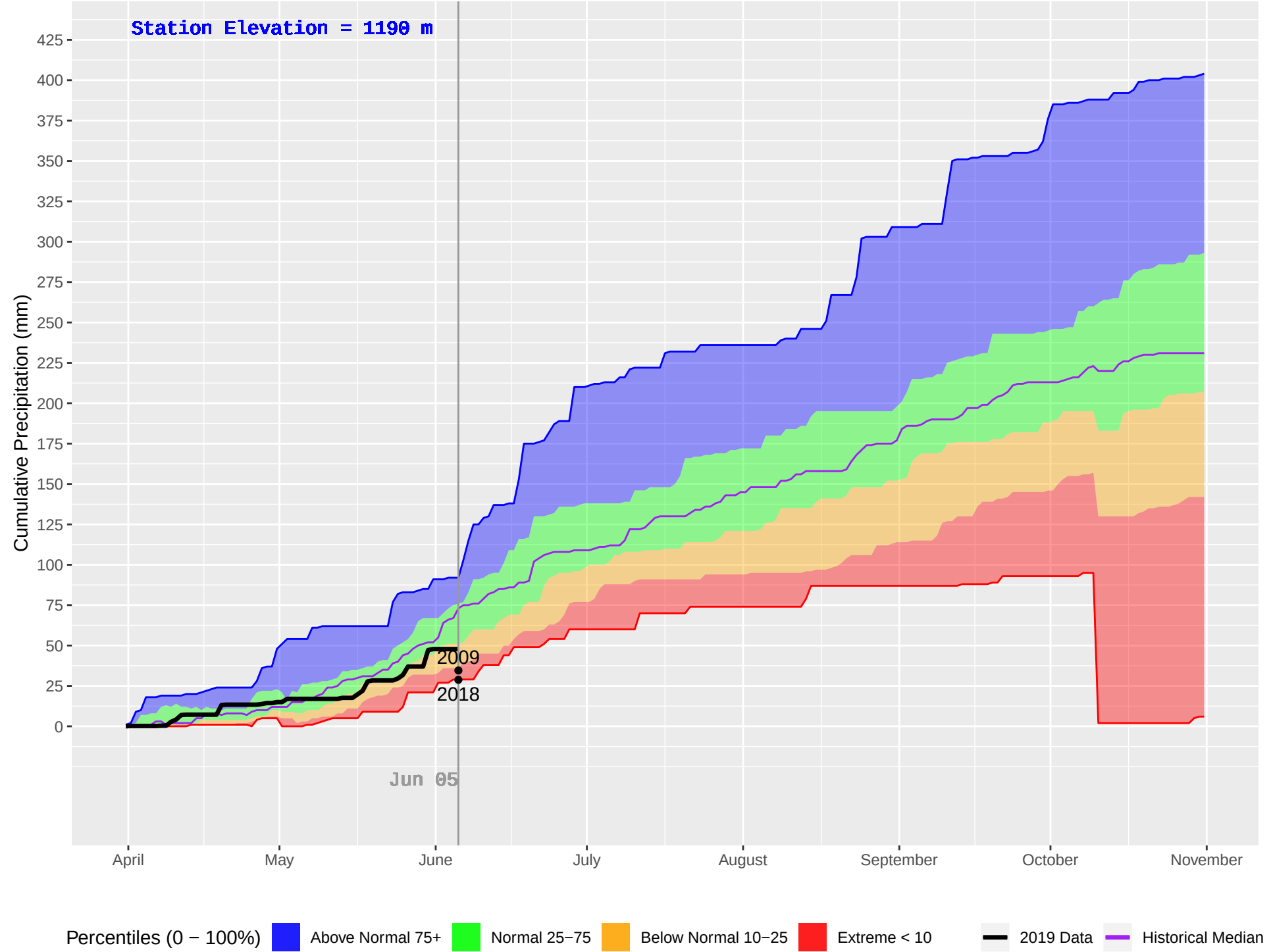
EMILY CREEK (425) : Historical (2002–2018), Current (2019) Daily Cumulative Precipitation
