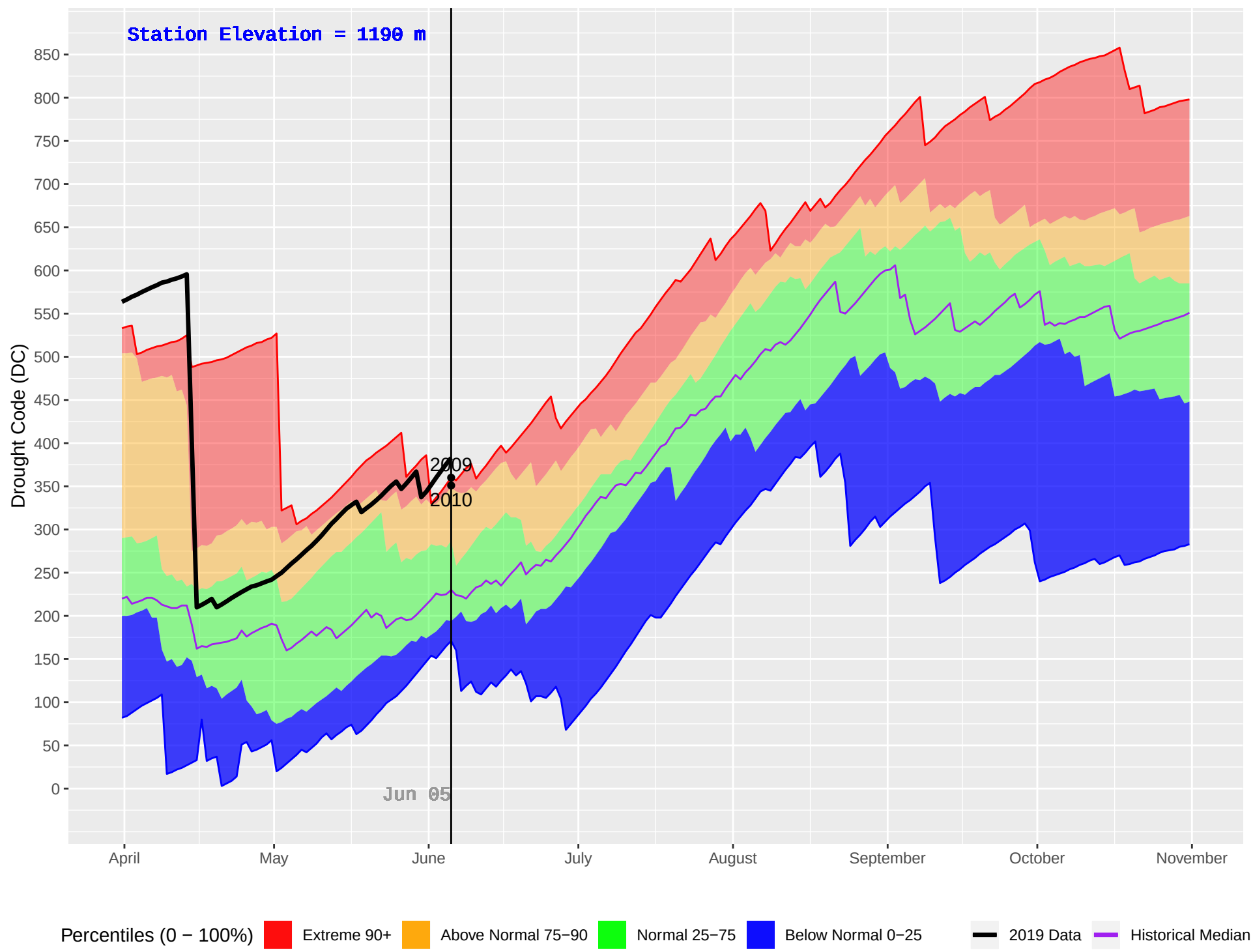
EMILY CREEK (425) : Historical (2002–2018) and Current (2019) Daily Drought Code (DC)
