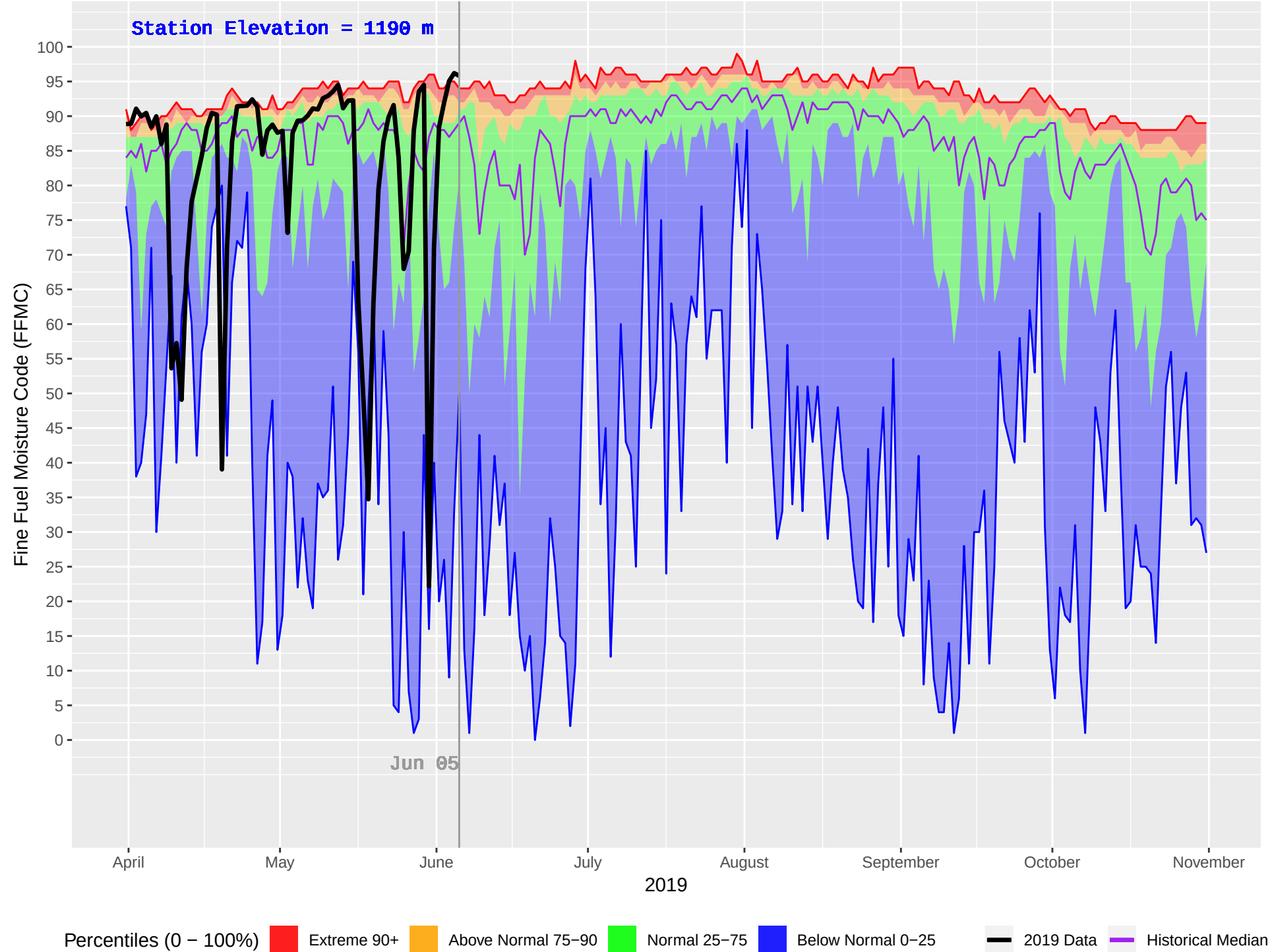
EMILY CREEK (425) : Historical (2002–2018) and Current (2019) Daily Fine Fuel Moisture Code (FFMC)
