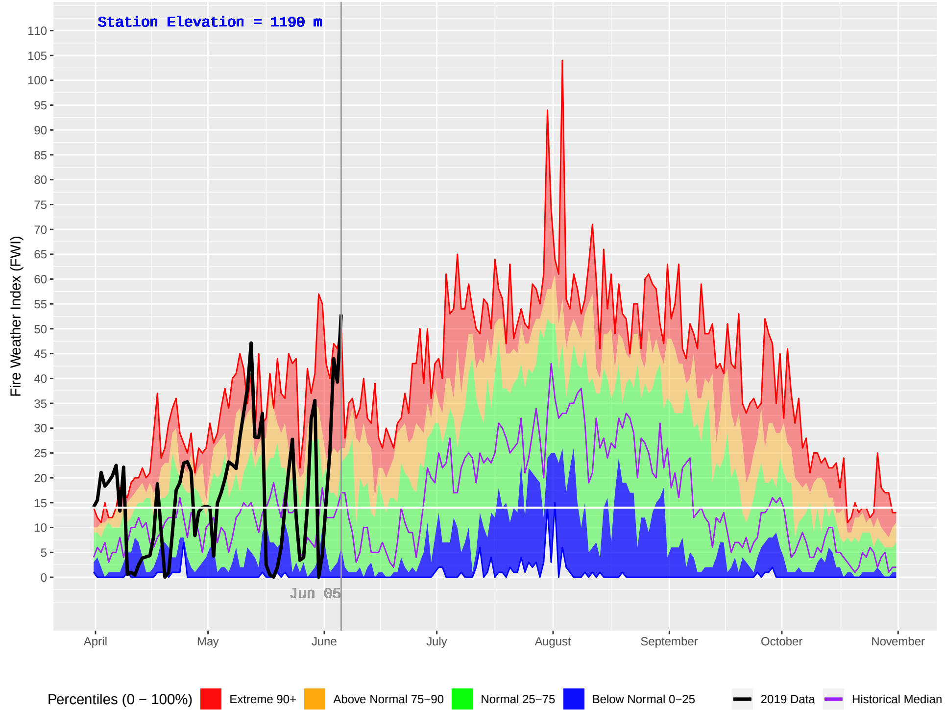
EMILY CREEK (425) : Historical (2002–2018) and Current (2019) Daily Fire Weather Index (FWI)
