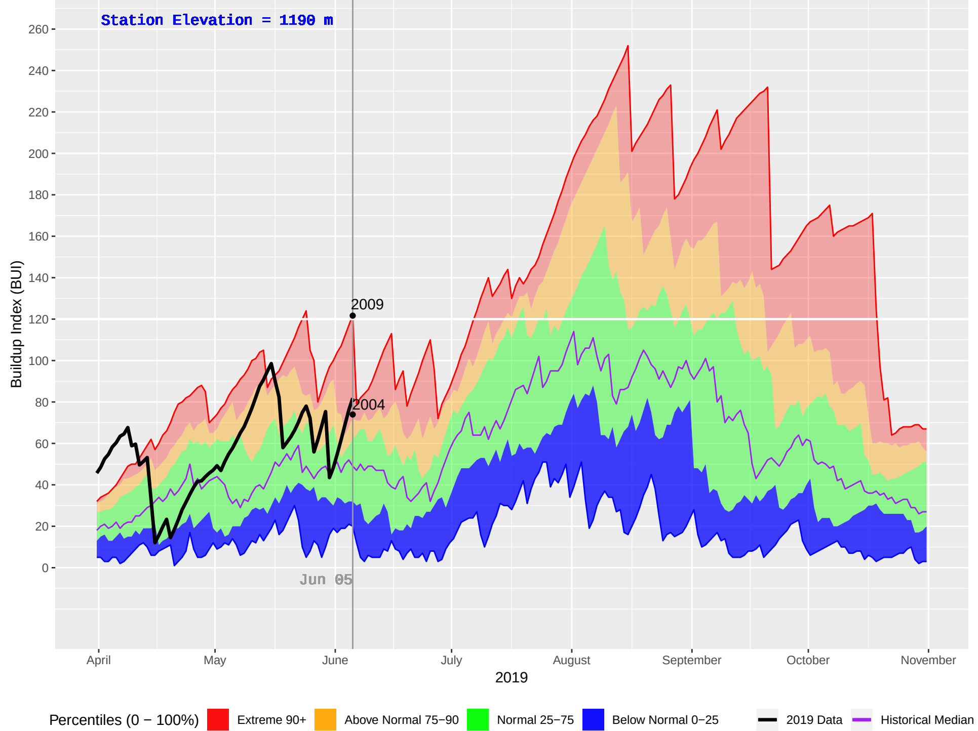
EMILY CREEK (425) : Historical (2002–2018), Current (2019) Daily Buildup Index (BUI)
